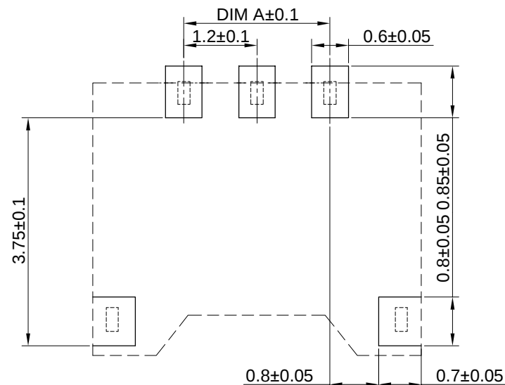
PCB LAYOUT
