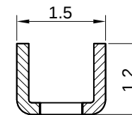
SEC:C-C
